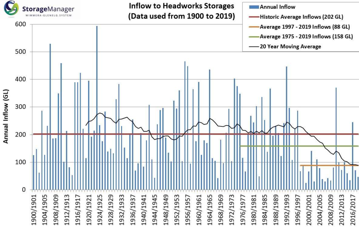
Figure 9 Annual inflows to GWMWater headworks storages (Source: Grampians Wimmera Mallee Water)
