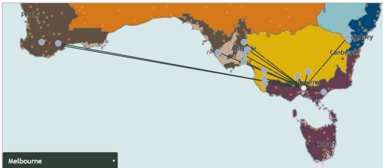
Figure 37 Climate Analogues for Melbourne for a 1 degree warming and 10% reduction in annual rainfall
