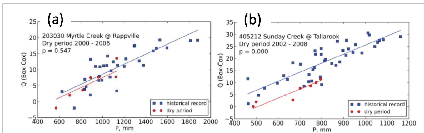
Figure 50 Box-Cox transformed annual runoff (Q) versus annual precipitation (P) for a 7 year dry period during the Millennium Drought relative to the historical record for two catchments (a and b) from Saft et al. (2015)
