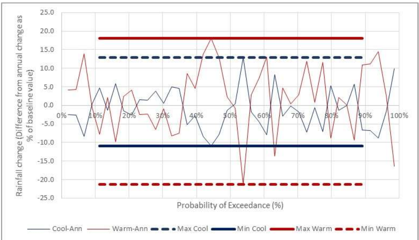
Figure 42 Maximum range of paired cool/warm season rainfall projections for the 10 th to 90 th percentile annual projections
