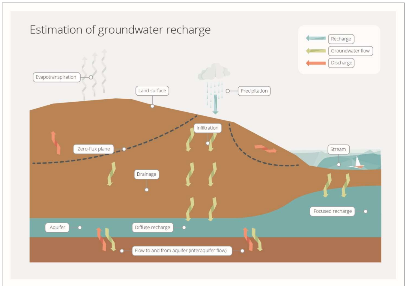
Figure 51 Conceptual diagram showing diffuse and focused recharge processes
