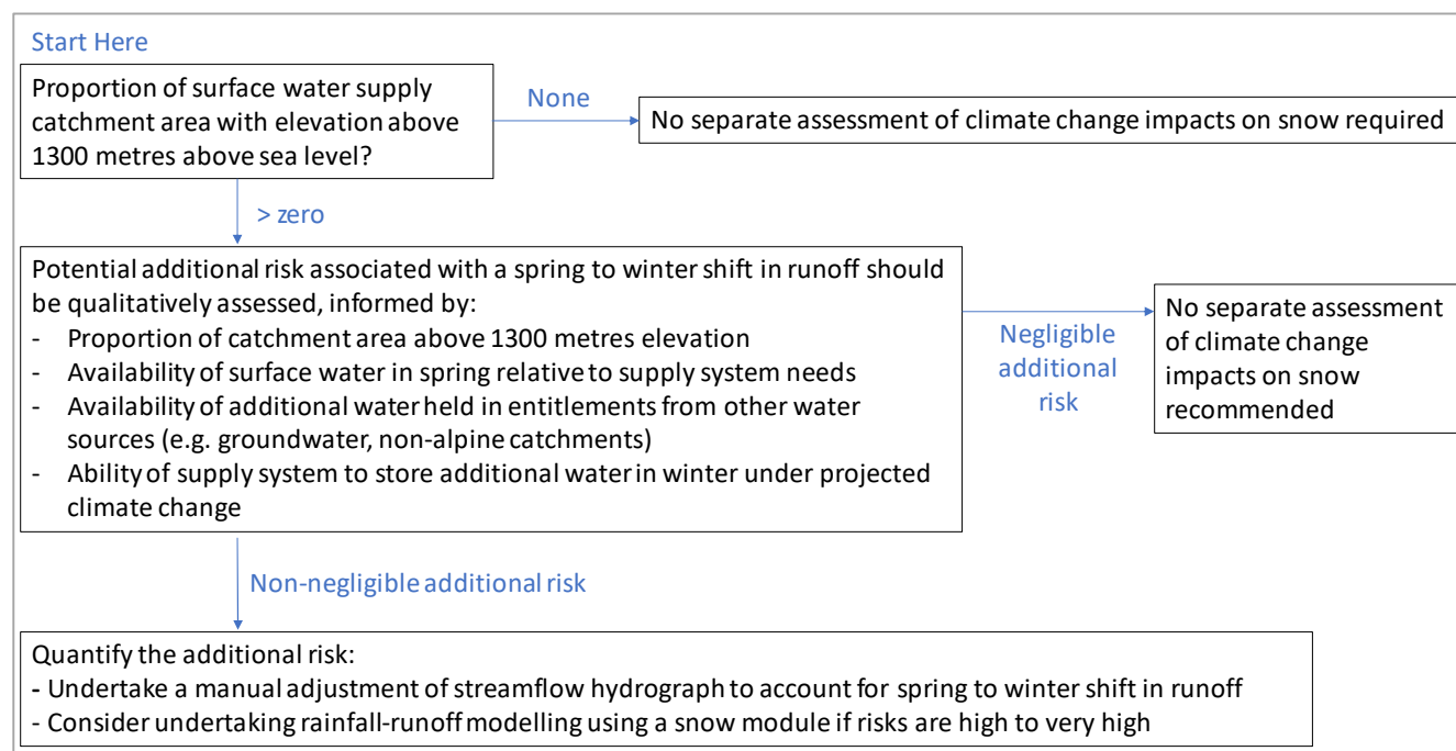
Figure 48 Decision process for assessing the potential risk associated with projected changes in snowfall, snowpack and snowmelt
