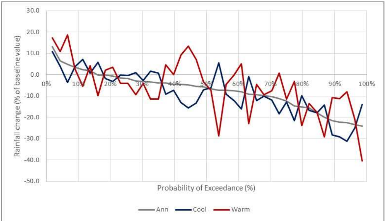
Figure 41 Cool and warm season projection variability by annual projected change for an example river basin, RCP and time slice
