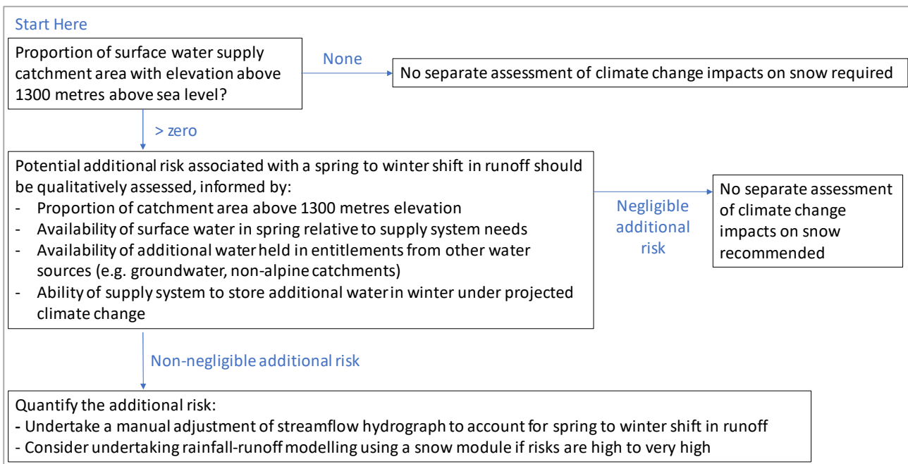
Figure 26 Decision process for assessing the potential risk associated with projected changes in snow cover
