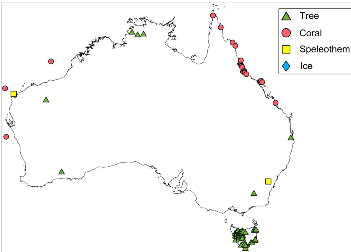
Figure 38 Availability of natural archives for use in paleoclimate reconstructions (Source: presentation by Ballis, 2019)
