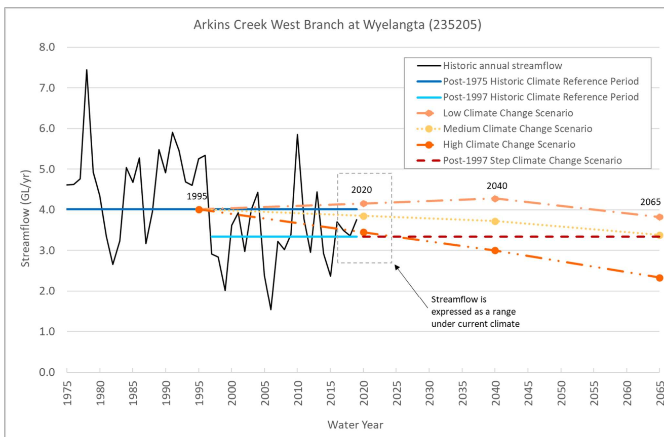
Figure 16 Example application of climate reference period and climate change scenario nomenclature illustrating projected changes in average streamflow conditions at a streamflow monitoring site in the Otway Coast Basin.
