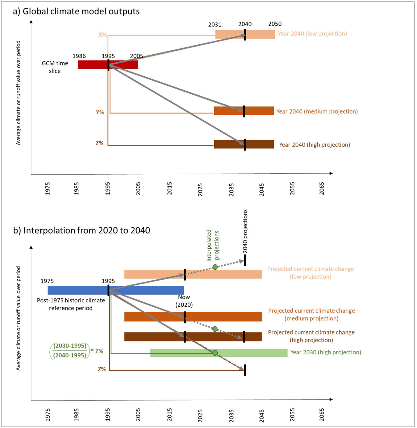
Figure 19 Interpolation of global climate model projections between 2020 and 2040
