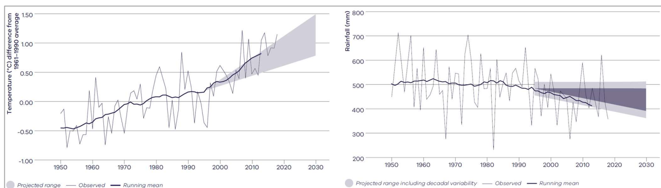
Figure 12 Comparison of observed annual temperature (left) and April to November rainfall (right) for Victoria relative to GCM projections (shaded area) for all emissions scenarios (DELWP, 2019d). Bold line is a running twenty-year average of observations.
