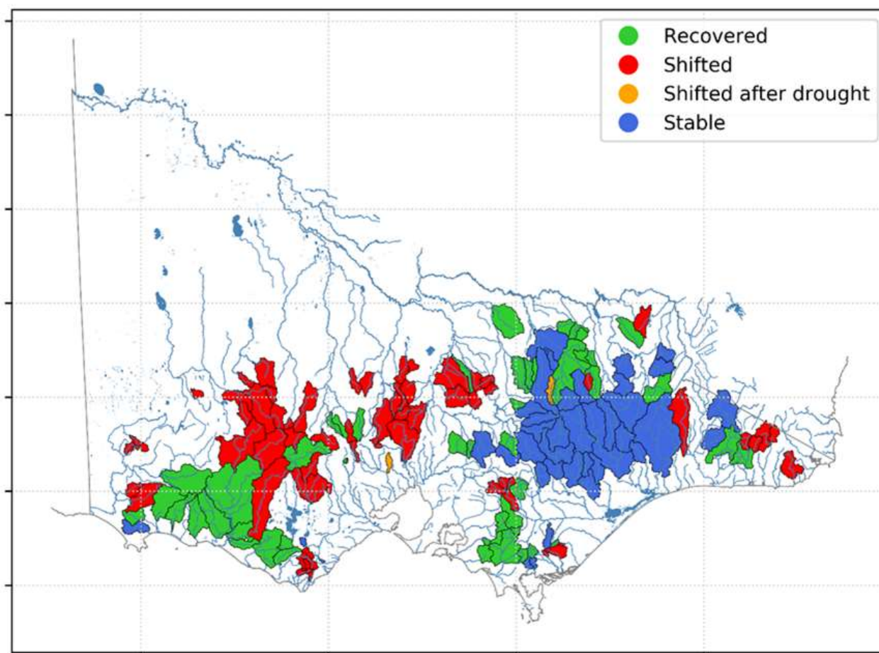
Figure 23 Shift in catchments hydrological response and recovery across Victorian catchments during and after the Millennium Drought. [Source: The University of Melbourne]
