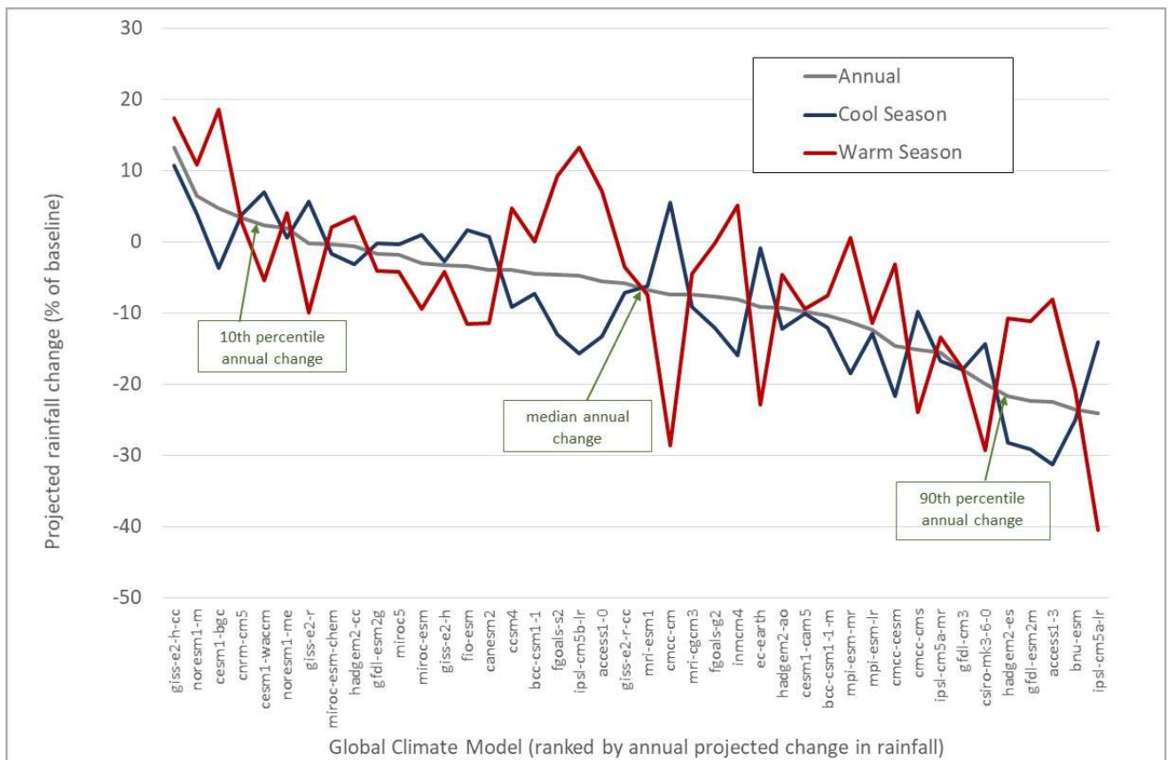
Figure 14 Projected change in cool and warm season rainfall for the Werribee Basin by ranked global climate model, RCP8.5 for the year 2065 (Source: data provided by CSIRO in 2020, based on analysis for Potter et al, 2016).
