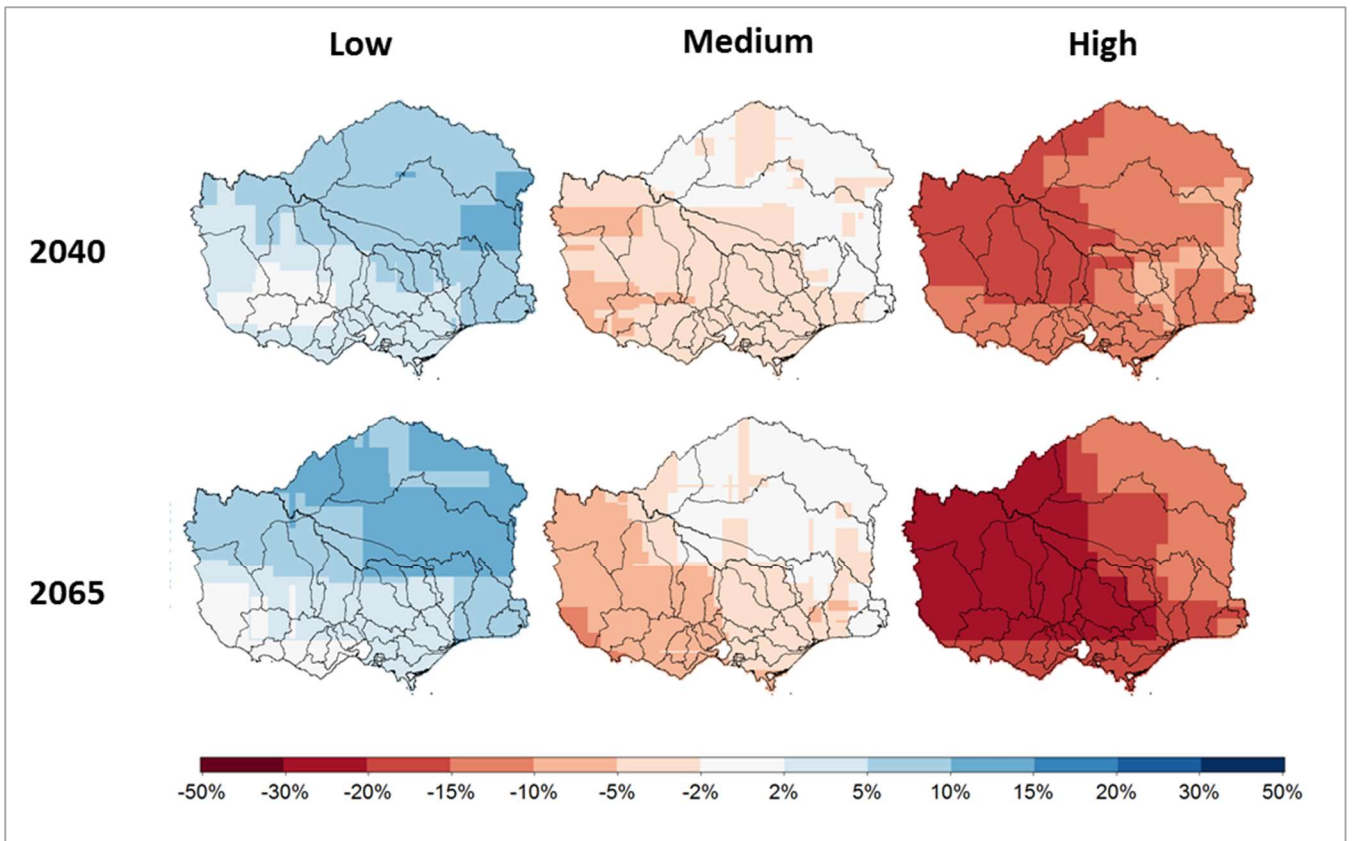
Figure 35 Projected changes in annual rainfall under emissions scenario RCP8.5 relative to current climate at a finer spatial scale (Source: Potter et al., 2016)
