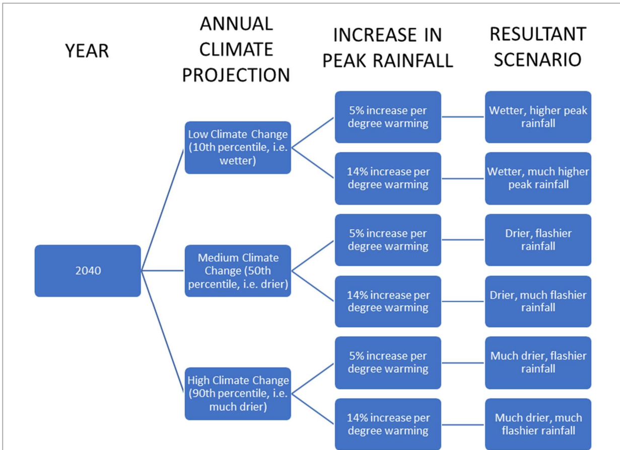
Figure 46 Plausible scenarios of 2040 water availability, coupled with increases in peak sub-daily rainfall
