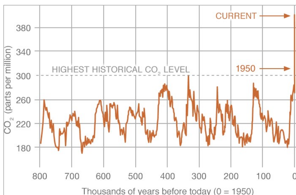
Figure 6 Trends in global atmospheric carbon dioxide over the last 800,000 years (NASA, 2020)
