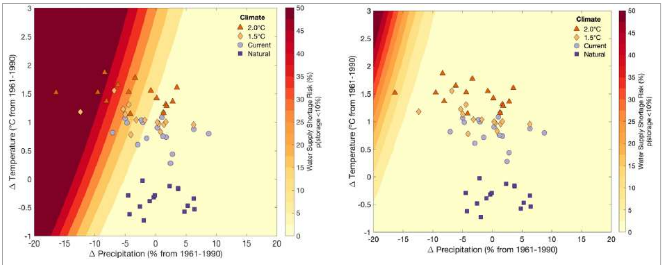
Figure 43 Changes in notional risk of water supply shortage under different levels of global warming without (left) and with (right) the Victorian Desalination Project (Henley et al., 2019)
