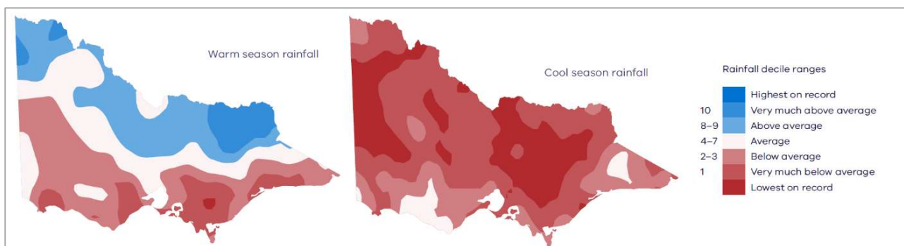
Figure 8 Observed rainfall in Victoria for the last 30 years (1989/90-2018/19) for the warm season (Nov-Mar) and cool season (Apr-Oct) relative to all other 30 year periods in the historical record (source: Bureau of Meteorology in DELWP (2019d)).
