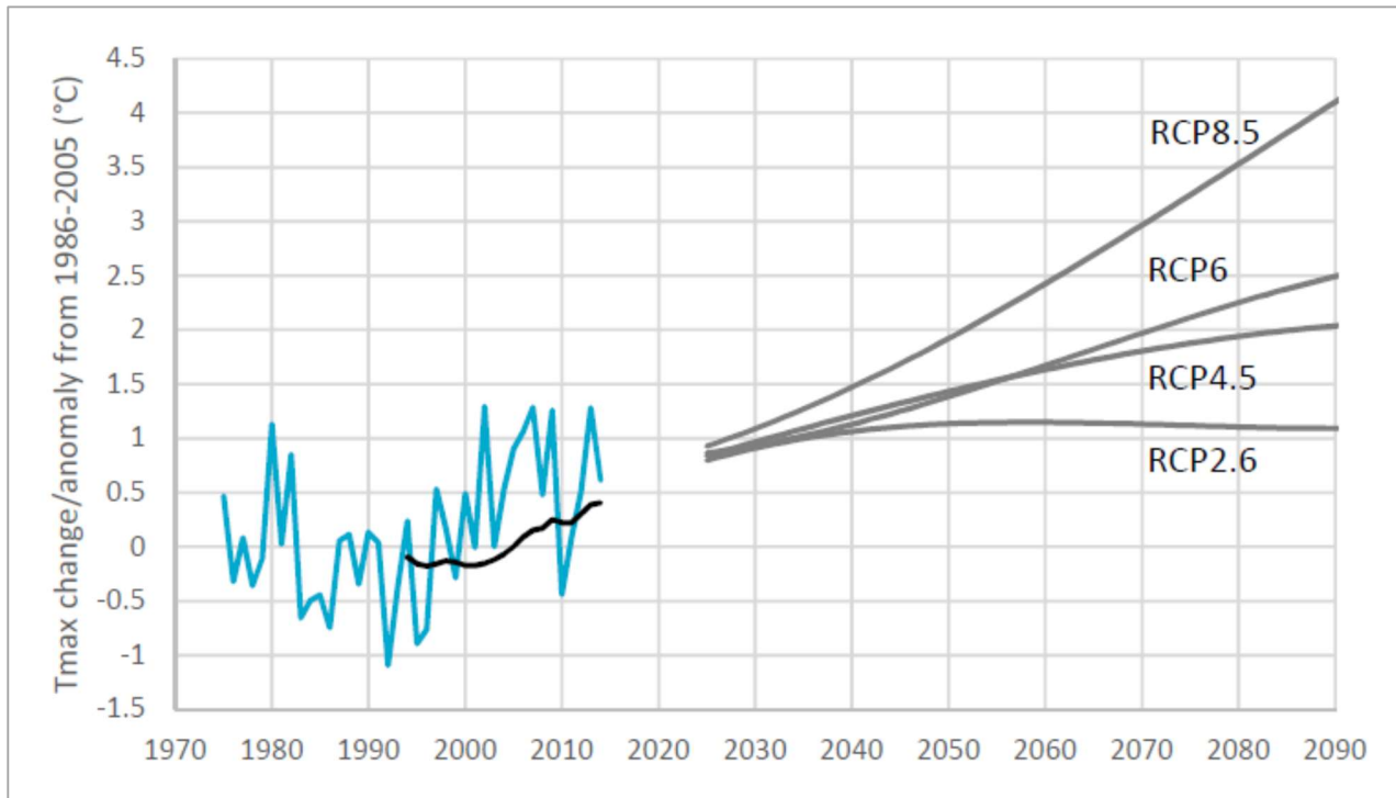
Figure 11 Temperature projections across the whole of the Murray-Darling Basin (Potter et al., 2016). Observations are shown in blue with a 20-year trailing moving average shown in black (i.e. the last value of the black line represents the average of the last twenty years of the blue line).
