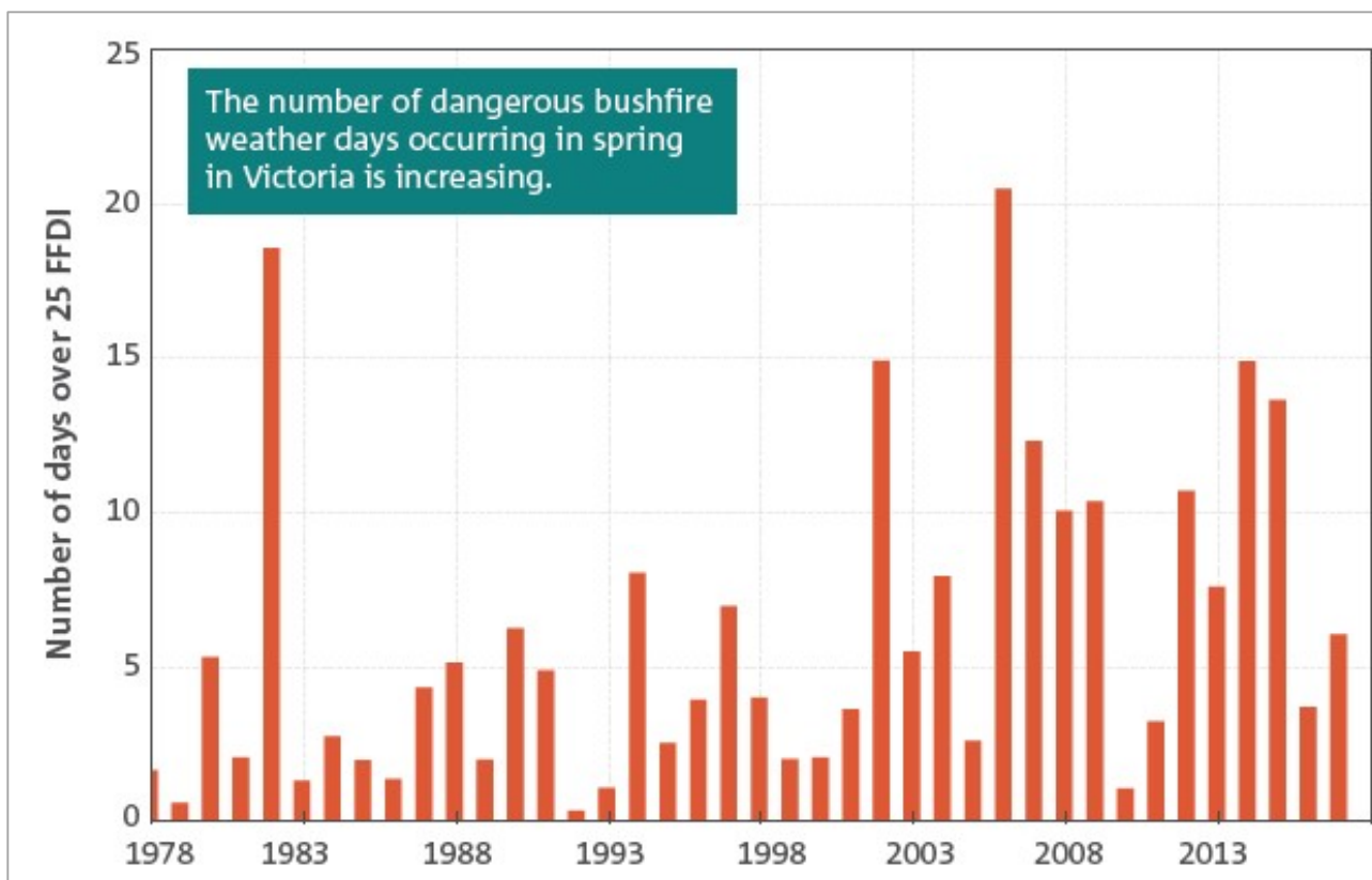
Figure 27 Number of dangerous bushfire days (forest fire danger index > 25) in spring in Victoria from 1978 to 2017 (Bureau of Meteorology and CSIRO, 2018)
