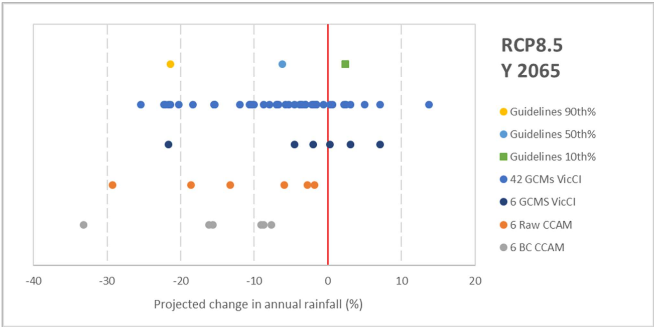
Figure 32 Werribee Basin comparison of VicCI and VCP19 (CCAM) rainfall projections 2065
