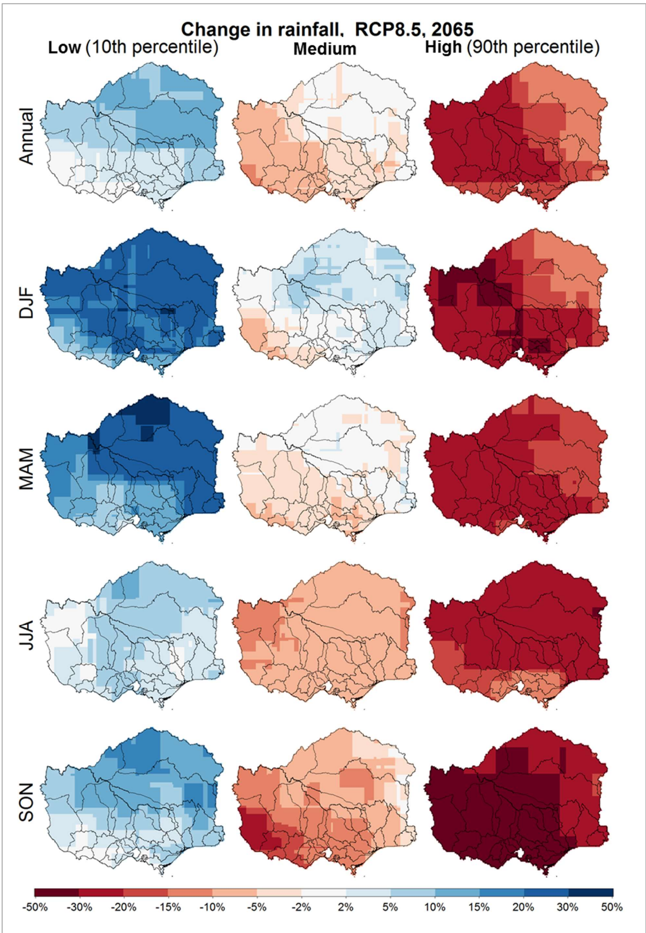
Figure 20 Projected changes in seasonal rainfall under emissions scenario RCP8.5 by 2065 relative to 1995 climate for study region, outlines correspond to Australian river basins (Source: Potter et al., 2016)
