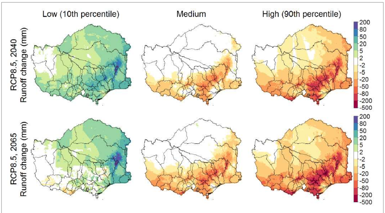
Figure 36 Projected changes in annual runoff under emissions scenario RCP8.5 relative to current climate at a finer spatial scale (Source: Potter et al., 2016)
