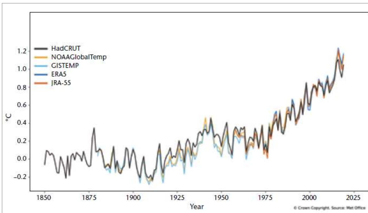
Figure 7 Global annual temperature anomaly relative to pre-industrial (1850-1900) levels, from three observed and two re-analysed datasets (WMO, 2020)
