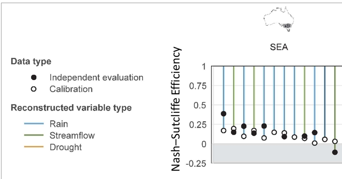
Figure 39 Quality of paleoclimate rainfall and streamflow reconstructions for south-east Australia (Source: Ballis, 2019)
