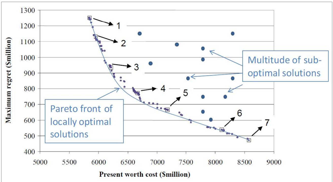
Figure 44 Example two-dimensional Pareto Front (Adapted from Cui and Kuczera, 2010)
