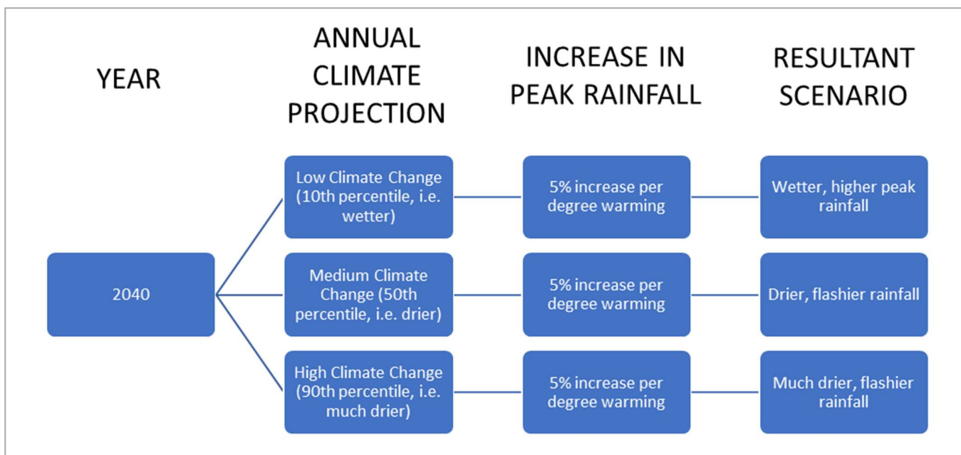
Figure 22 Plausible scenarios of 2040 water availability, coupled with increases in peak daily rainfall.
