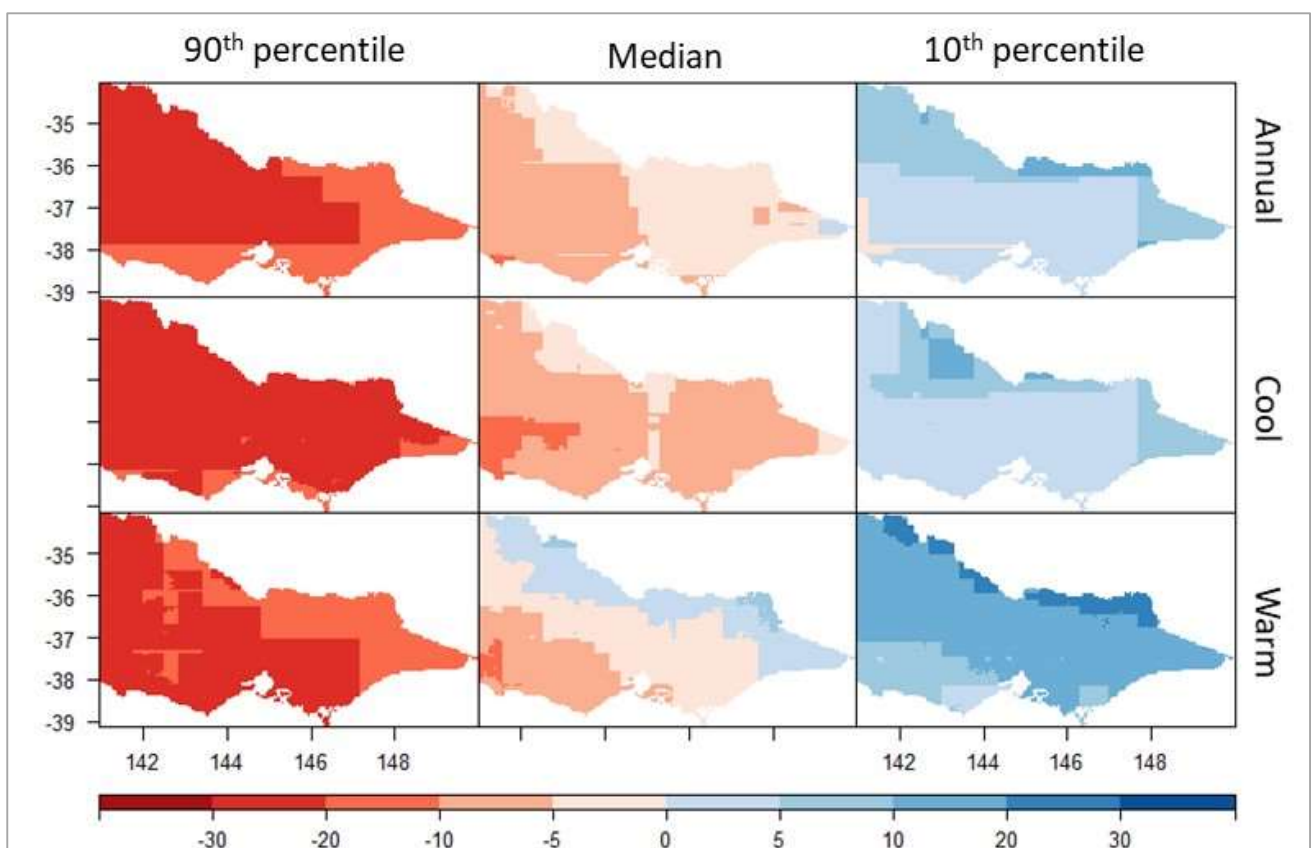
Figure 13 Projected 10 th , 50 th and 90 th percentile cool and warm season rainfall changes (% change from 1995 value) across Victoria for RCP8.5 in the year 2065 (source: CSIRO)
