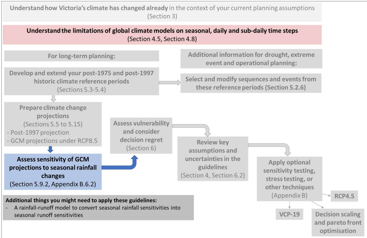
Figure 4 Overview of additional sections of high relevance for environmental water management
