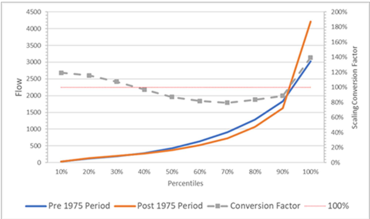
Figure 31 Example of low flow and high flow increases under historical data scaling (HARC, 2020a)
