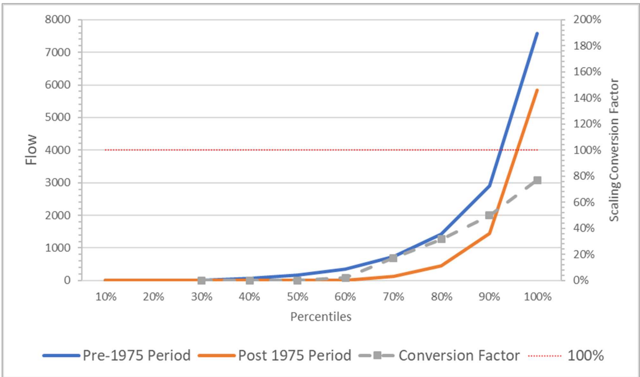
Figure 29 Example of expected historical data scaling, with post-1975 flows lower than pre-1975 flows in all deciles (HARC, 2020a)
