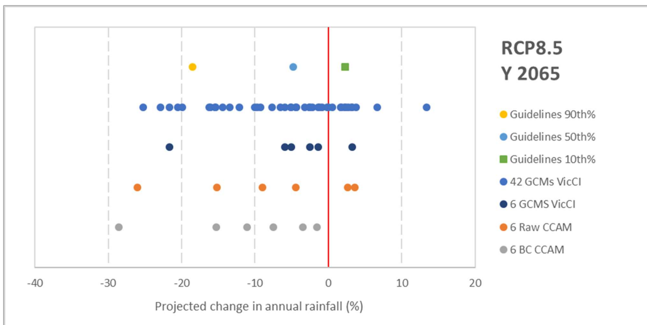
Figure 34 Mitchell Basin comparison of VicCI and VCP19 (CCAM) rainfall projections 2065
