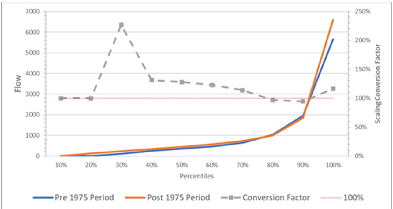
Figure 30 Example of anomalies historical data scaling (HARC, 2020a)
