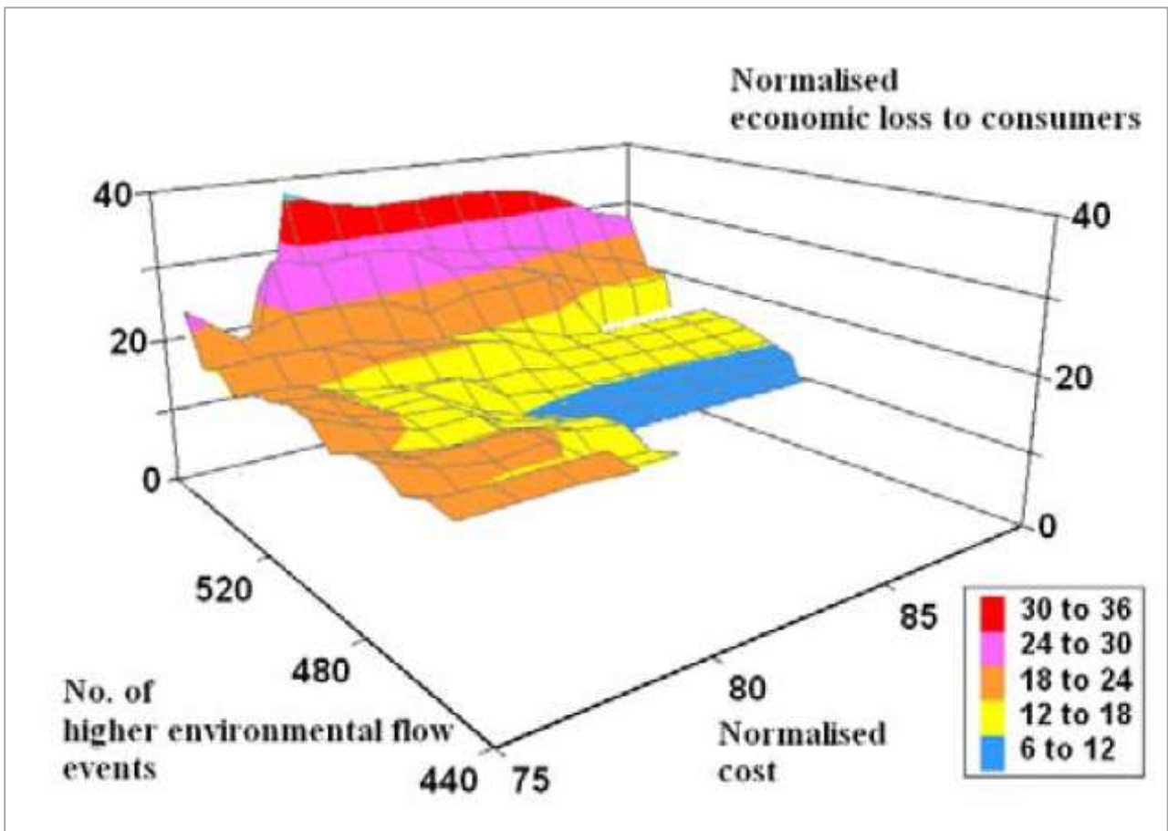
Figure 45 Example three-dimensional Pareto Front (Kularathna et al., 2015)
