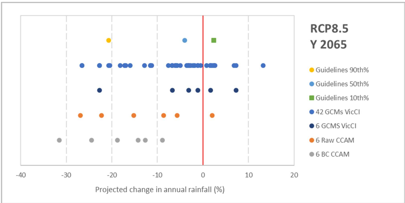
Figure 33 Goulburn Basin comparison of VicCI and VCP19 (CCAM) rainfall projections in 2065
