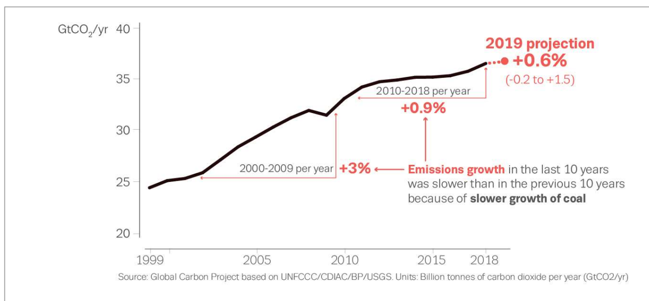
Figure 5 Recent Historical Growth in Carbon Dioxide Emissions from Fossil Sources, as estimated by the Global Carbon Project (GCP, 2020)
