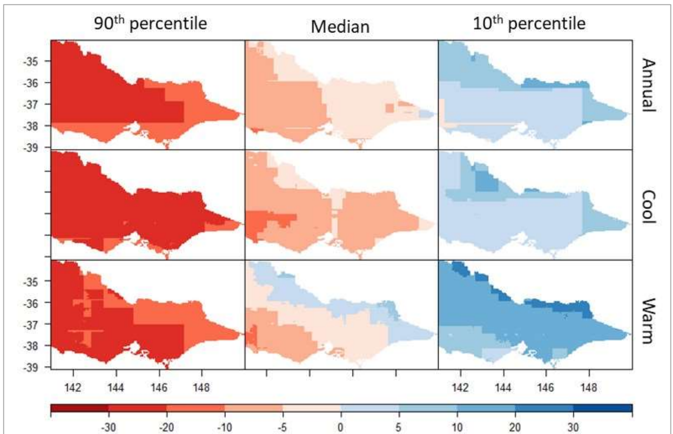
Figure 21 Projected 10 th , 50 th and 90 th percentile cool and warm season rainfall changes (% change from 1995 value) across Victoria for RCP8.5 in the year 2065 (source: CSIRO)
