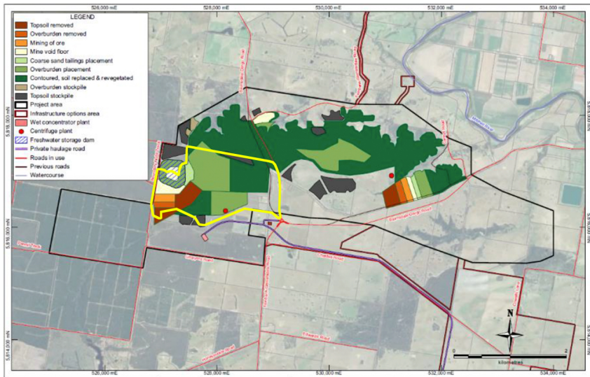
Figure 9-9: Disturbed and rehabilitated areas—Year 5 (indicative)
