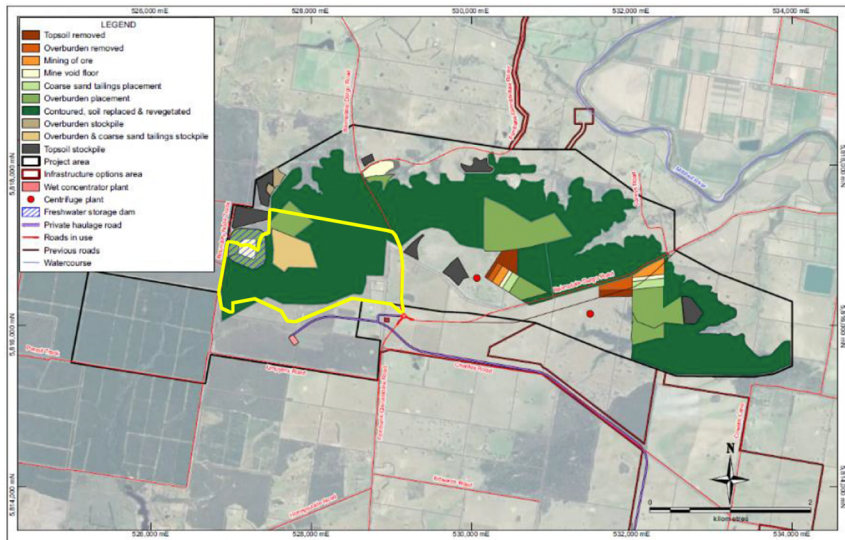
Figure 9-10: Disturbed and rehabilitated areas – Year 8 (indicative)
