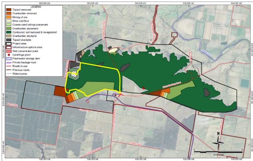
Figure 9-11: Disturbed and rehabilitated areas – Year 12 (indicative)
