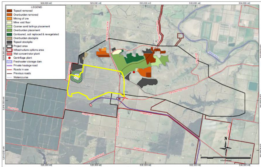
Figure 9-8: Disturbed and rehabilitated areas – Year 1 (indicative).
